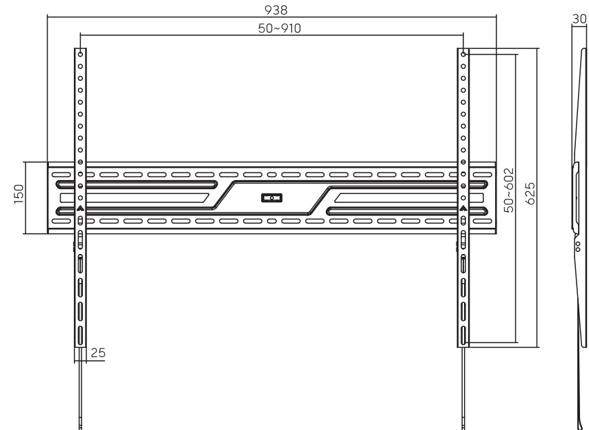
Dimensions (mm)
